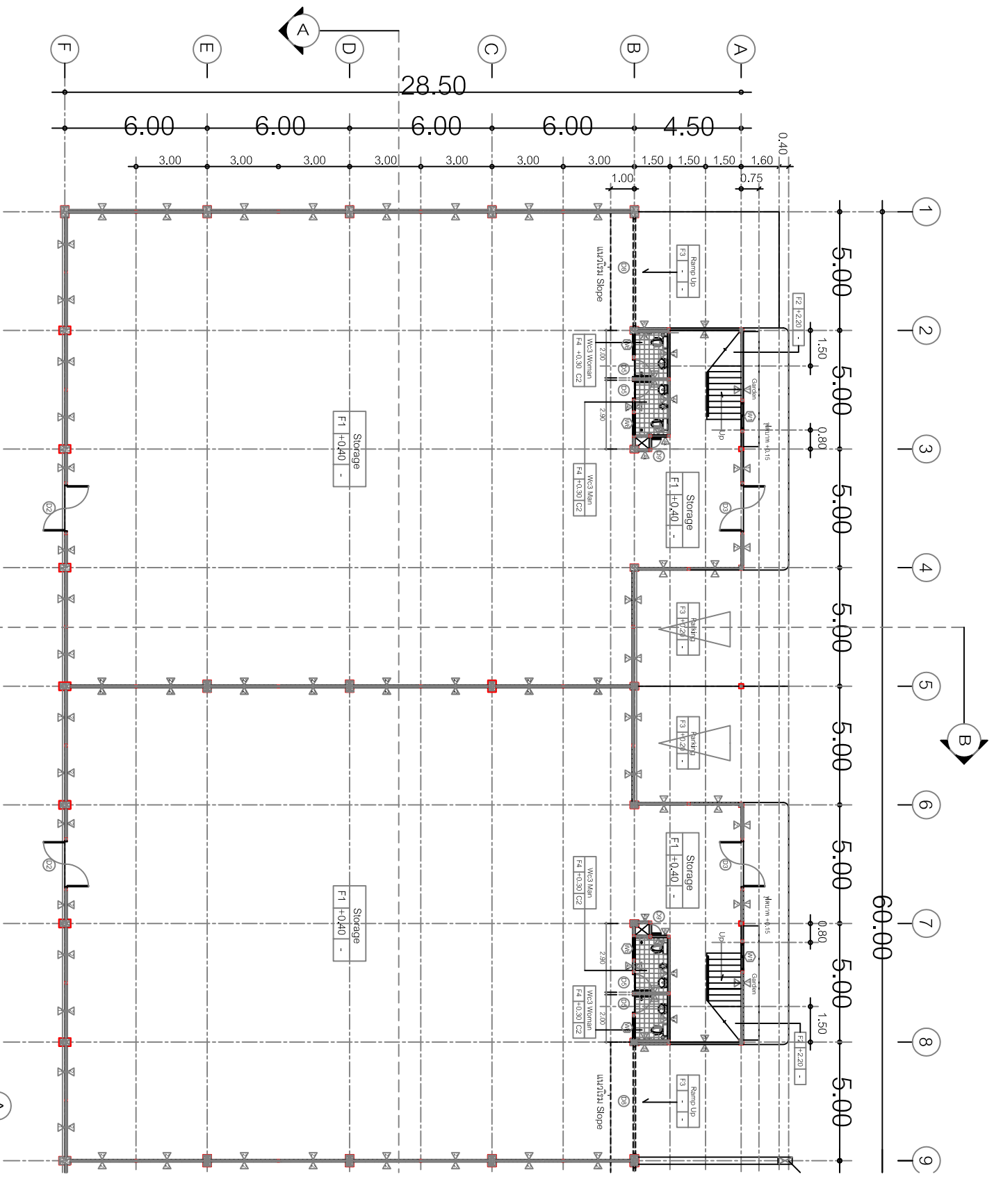
Plan Floor 1 Type B Scale 1:100
